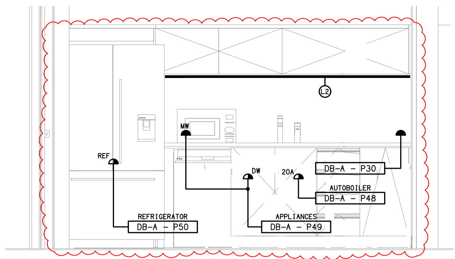
DETAIL A LUNCHROOM KITCHENETTE ELEVATION SCALE 1: 20
